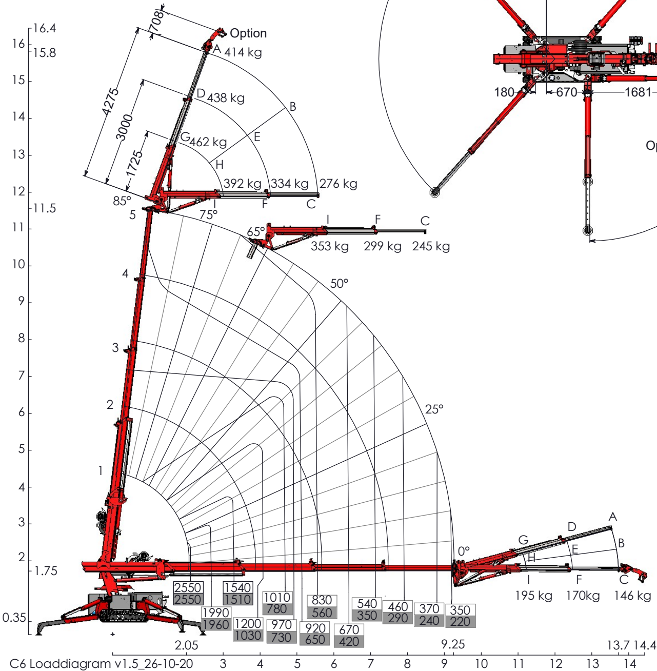
Loadchart C6 without counterweight
