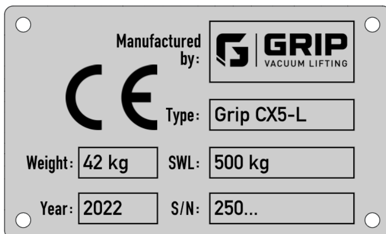
Figure 1: Nameplate
